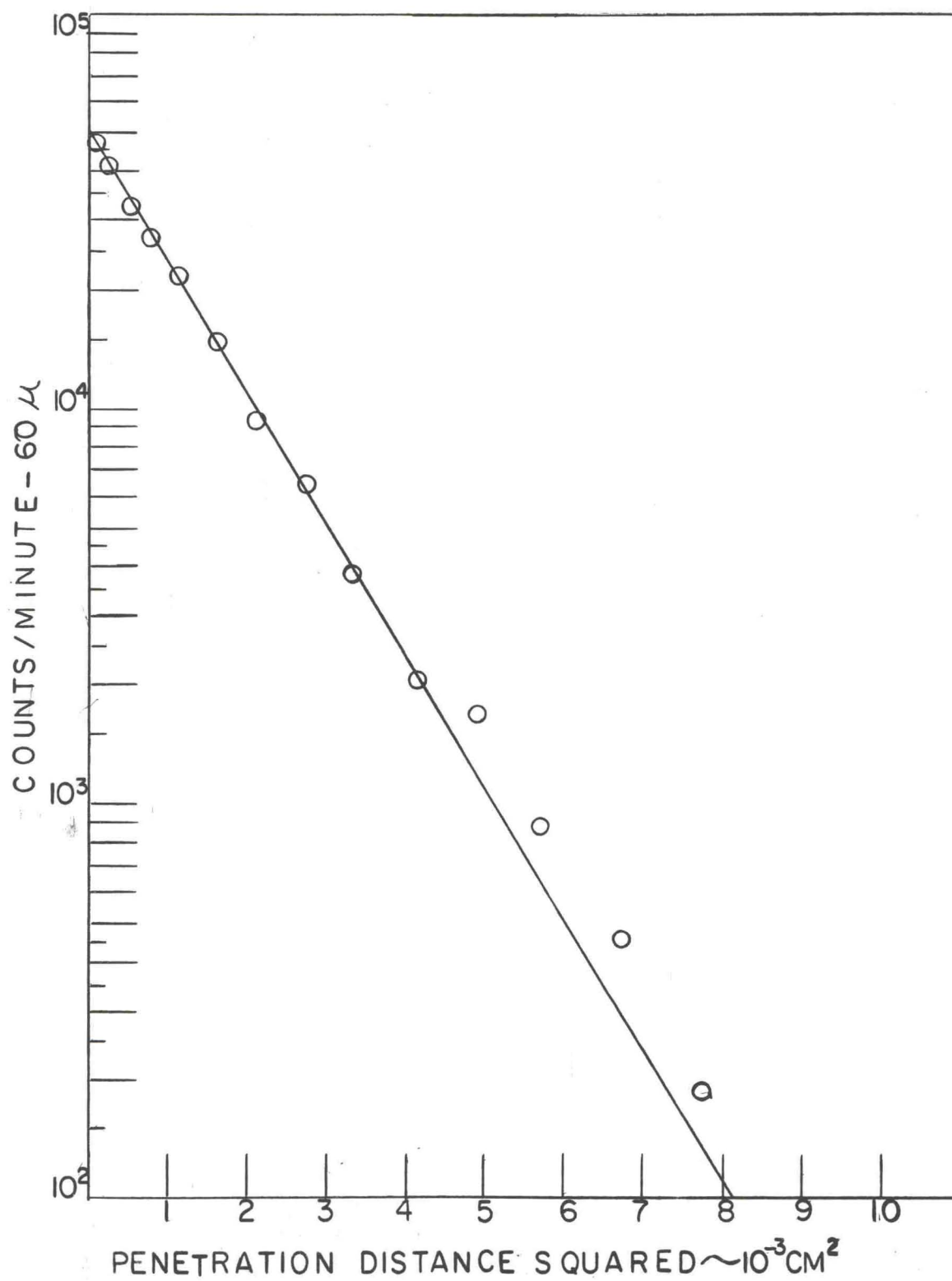
Figure 7. Solute Penetration Curve, Sample No. 77-- Annealed at 24 kb. pressure and 590°K for 5.13 \times 10^4 sec
